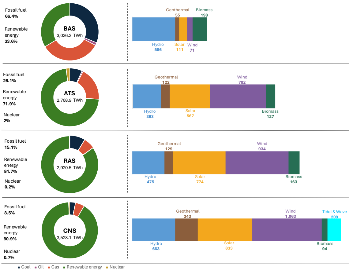
Figure 10. ASEAN Power Generation Across Scenarios
