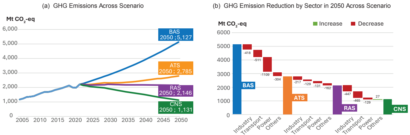
Figure 15. GHG Emissions in All Sectors Across Scenarios
